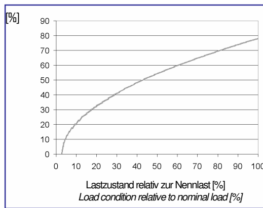
Emergency lowering device for JDN Winches
